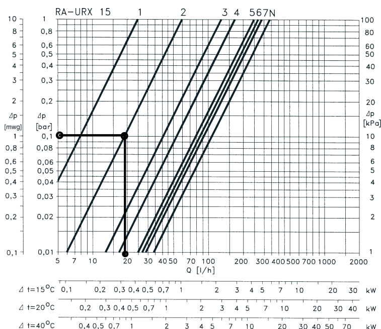
Capacity with RA-URX, RLV-X and RAX sensor at a P-band between 0.5 K and 2 K.
