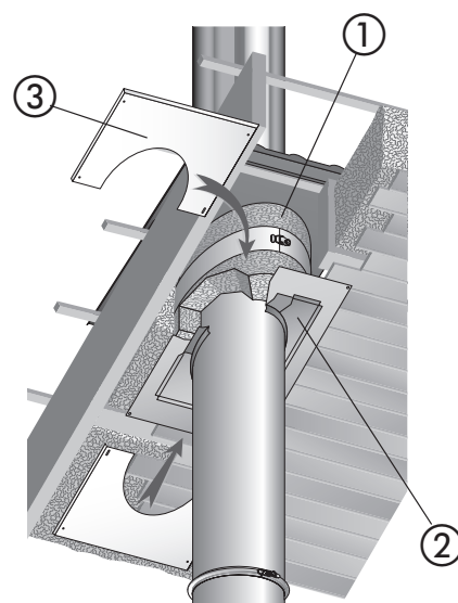
① COQISOL ② PDSER ③ PP PDSER
