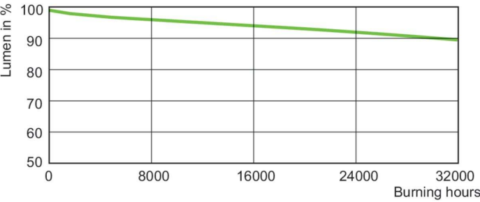
Lumen Maintenance Diagram - MASTER GreenPower CG T 400W E40
