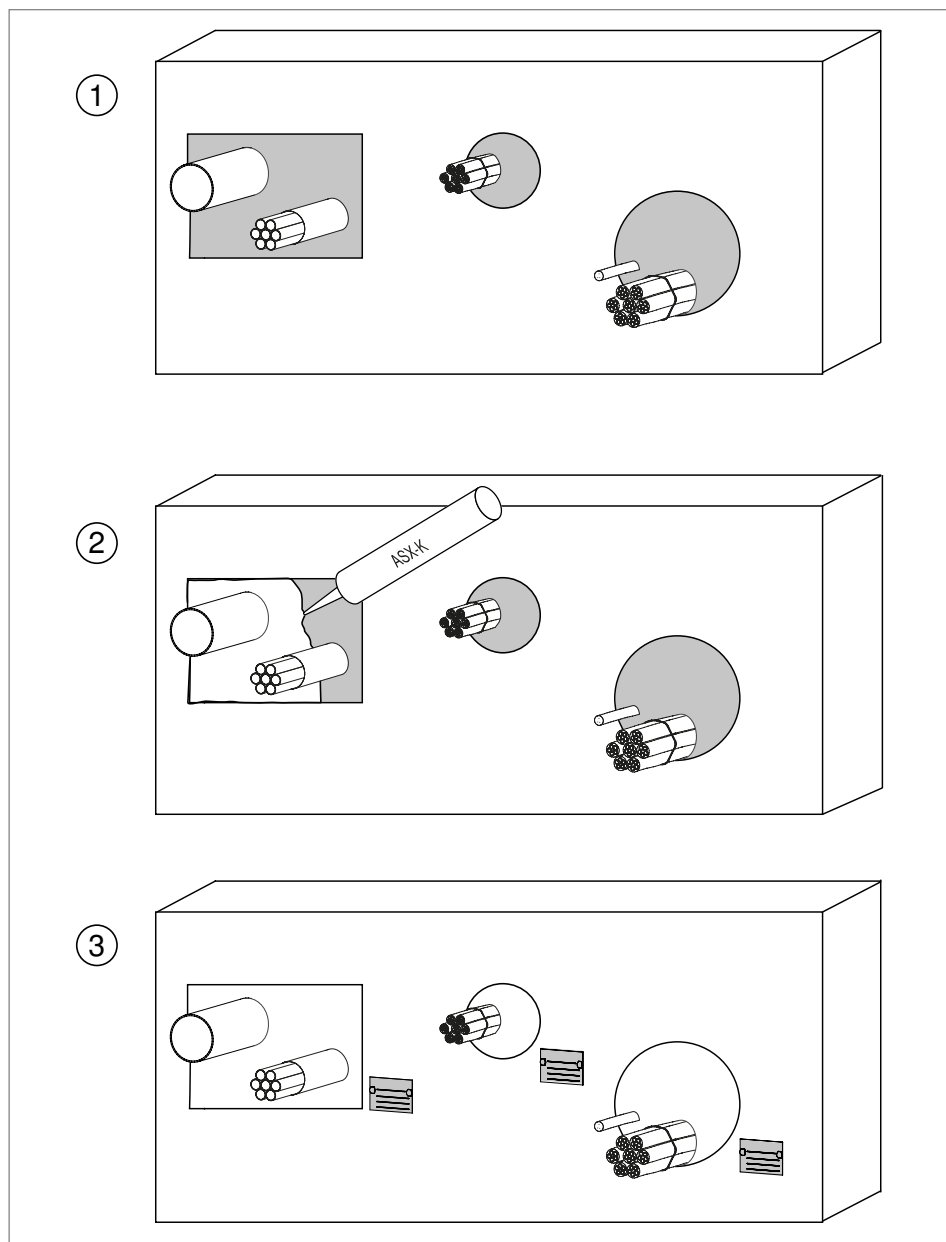
Fig. 10: Mounting small insulation
