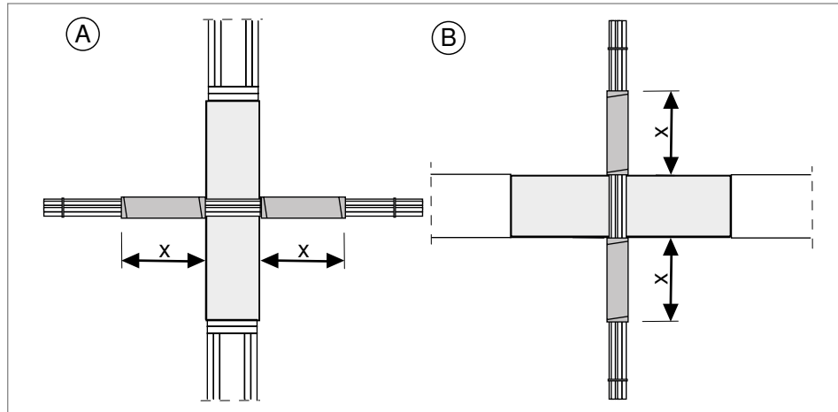
Fig. 4: Measure: FSB-WB 1.5 fire protection coil in wall A and ceiling B
