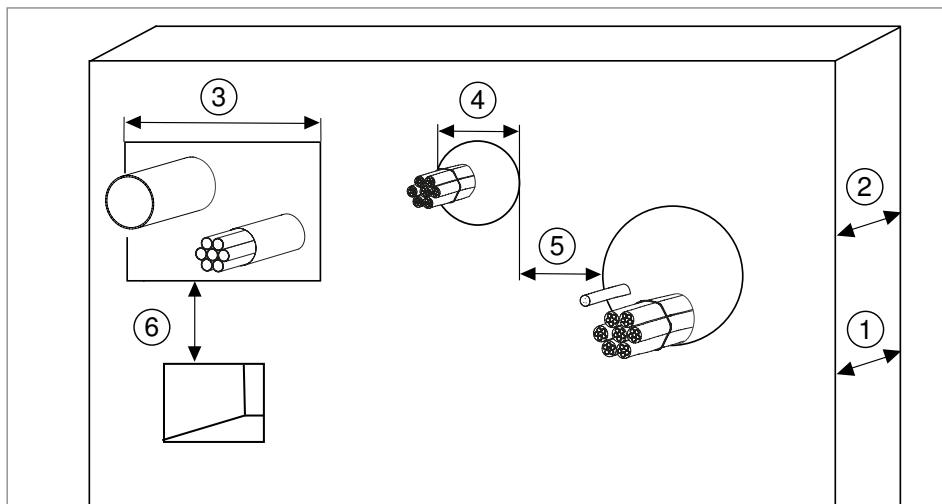
Fig. 2: Insulation distances to other components or component openings
