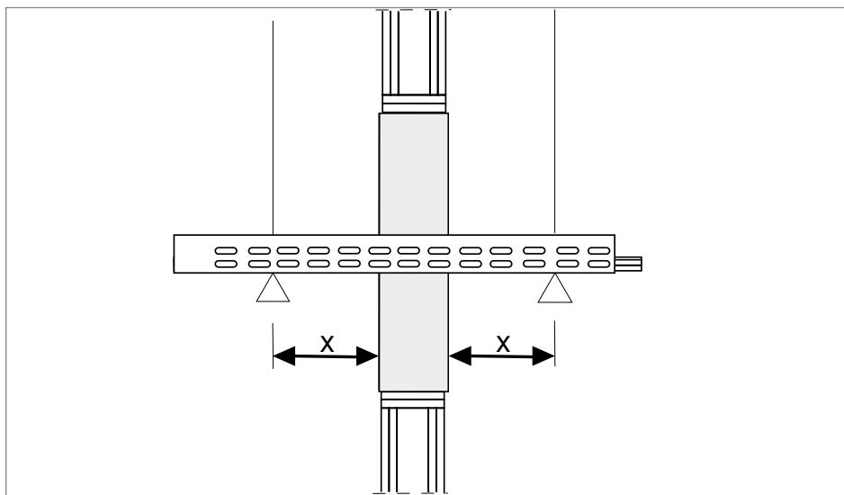
Fig. 3: Maximum distance for supports
