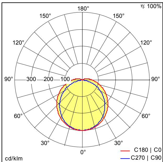
TE_JULIE_1500_LED_IP65_6300_840.idt
