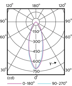
Light Distribution Diagram - MAS LED spot VLE D 4.9-50W GU10 930 36D
