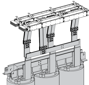
Flatwise with side in comer for Canalis KTA5000/KTC6300
