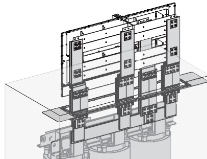
Edgewise with side in comer for Canalis KTA5000/KTC6300
