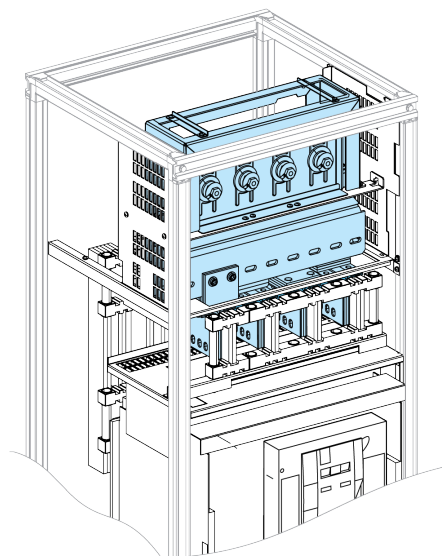
Okken switchboard
