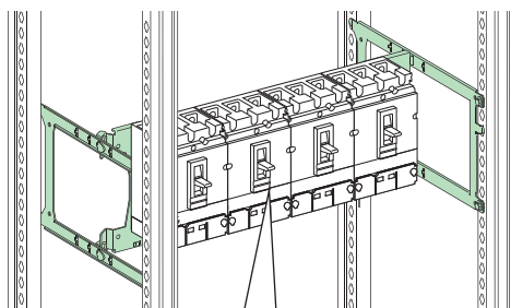
Compact NSX100/160/250 3P/4P Vigi NSX100/160/250 3P/4P
