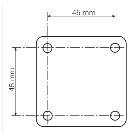
Fig. 2: Hole pattern.
