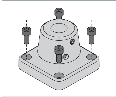
Fig. 1: Fastening element
