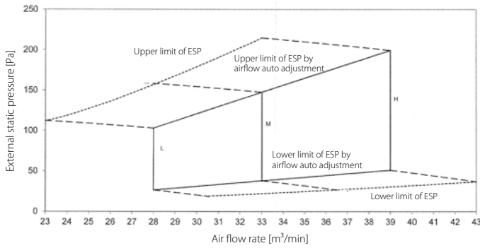
Fan characteristics (3) (airflow auto adjustment)
