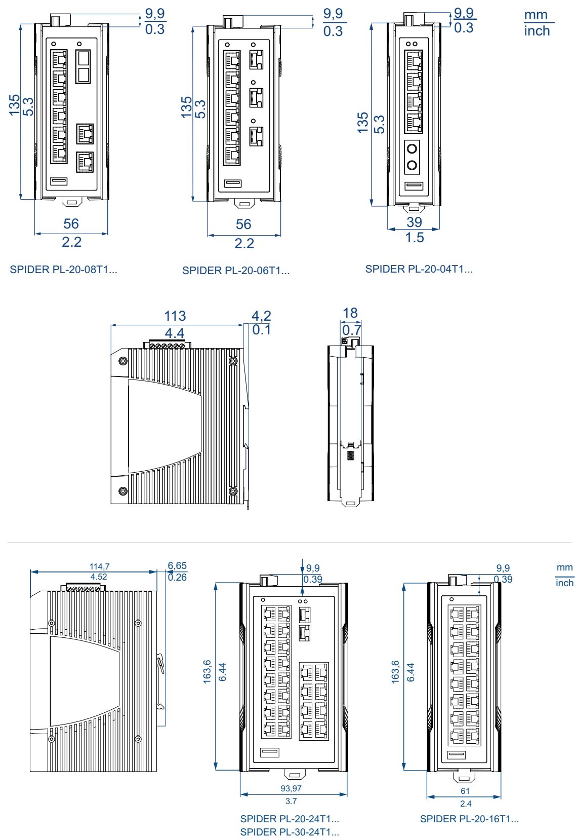
Figure 5: Dimensions of device variants SPIDER PL-20... and SPIDER PL-30...
