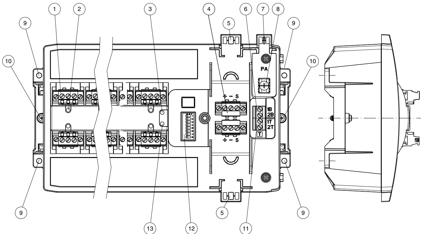
Figure 2: component overview
