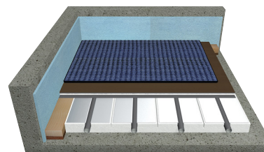
Constitution de plancher chauffant sec
