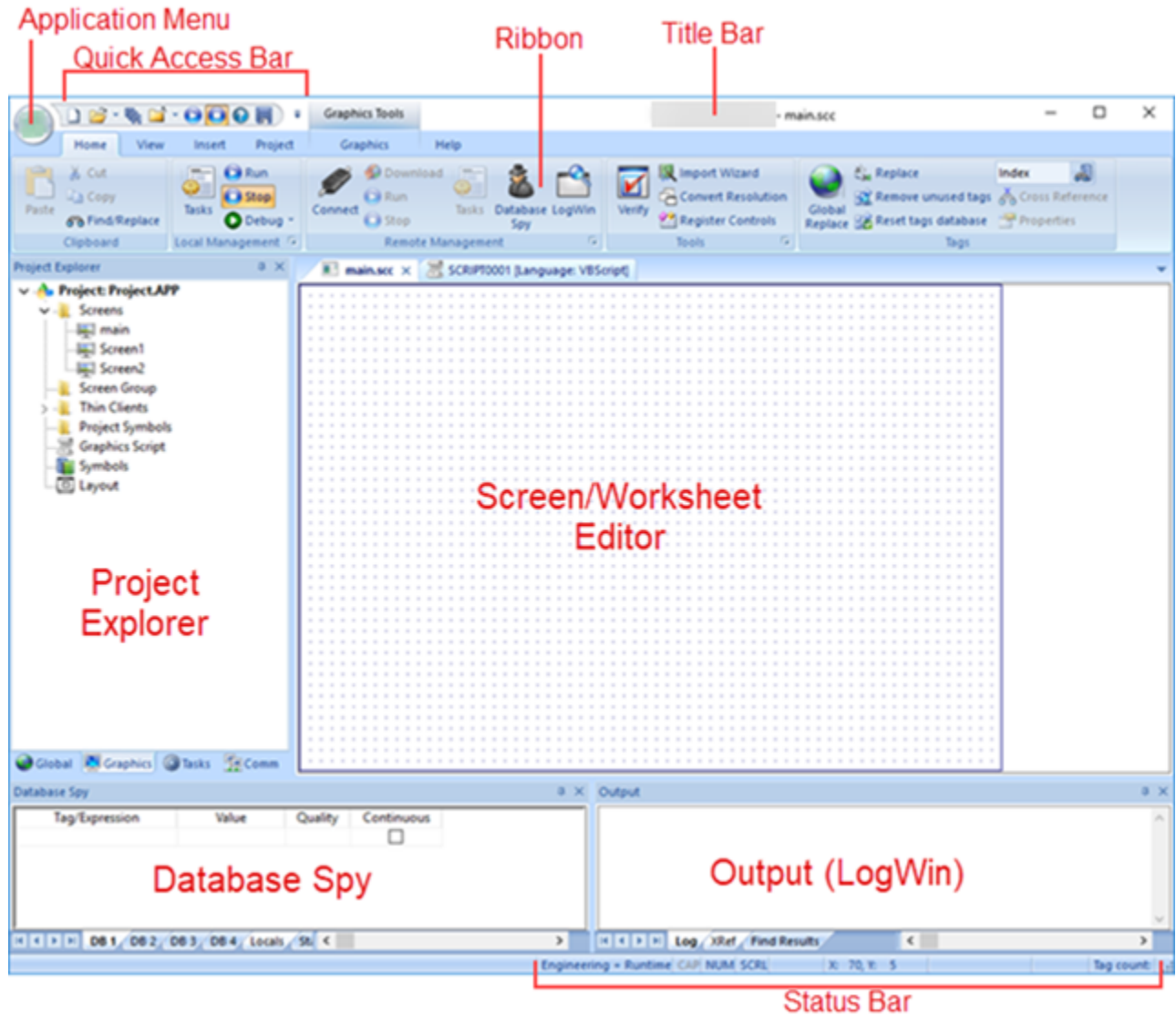
The EcoStruxure Machine SCADA Expert Development Environment
