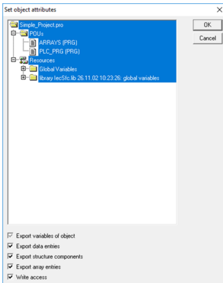
Clearing the options for all objects
