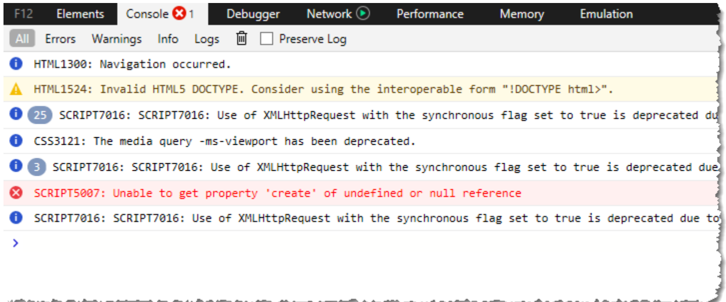
An example of the activity log in the Internet Explorer 11 console
