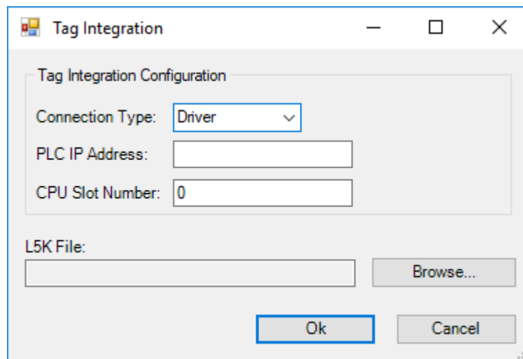
RSLogix Tag Integration dialog box
