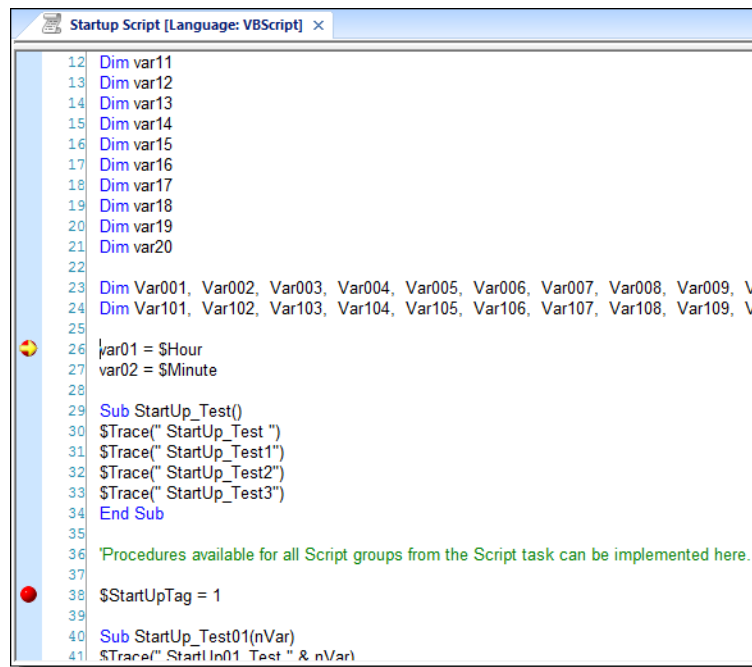
The yellow arrow shows where execution was suspended
