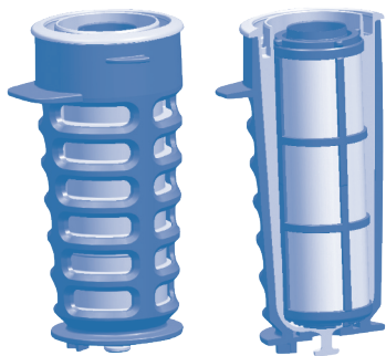
fig. 3 – Hygiejnisk filterhus (Filterhus + filterelement) i sort holder
