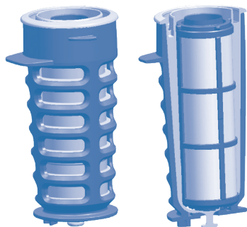
Fig. 3 – Hygienic vault (filter cup + filter element) in the black supporting core
