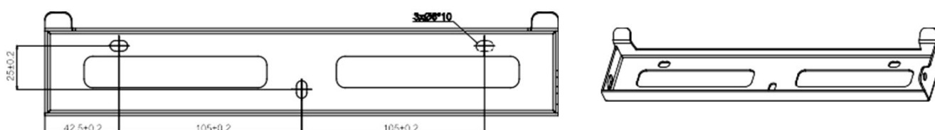
Figure 4 – Dimensions de l'étrier
