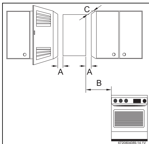
Fig. 17 Distances minimales
