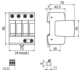
Dimensions DG M TNS ACI 275 FM
