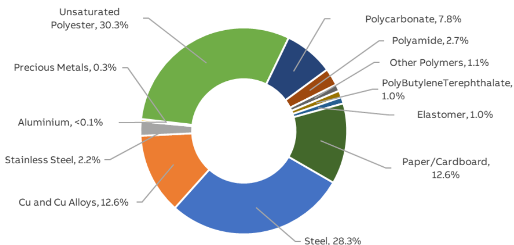
Figure 1: Composition of XT5 N/S/H/L 3P IEC TMA 400A
