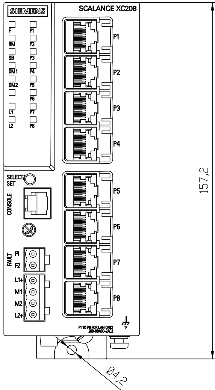
Vorne offen / Front open Alternative Befestigung / Alternative mounting
