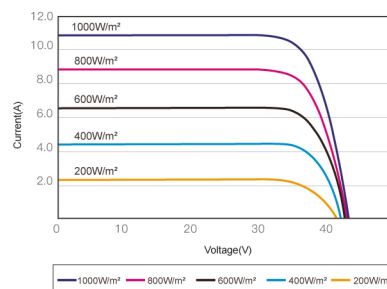
I-V CURVES OF PV MODULE(370W)
