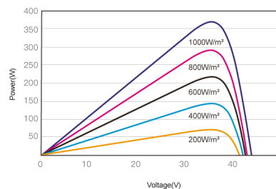
P-V CURVES OF PV MODULE(370W)
