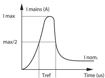
Inrush current
