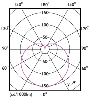
Light Distribution Diagram - CorePro LEDbulb ND 4.9-40W A60 E27 930
