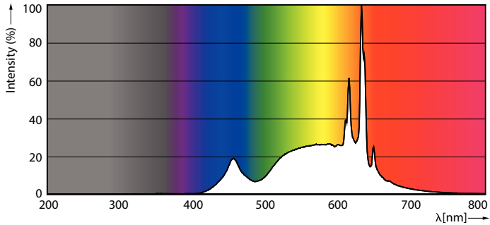
Spectral Power Distribution Colour - CorePro LEDbulb ND 10.5-75W A60 E27 930
