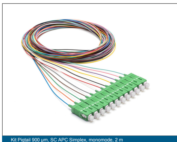
Kit Pigtail 900 \mu m, SC APC Simplex, monomode, 2 m
