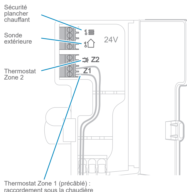
fig. 18 - Borniers TBTS
