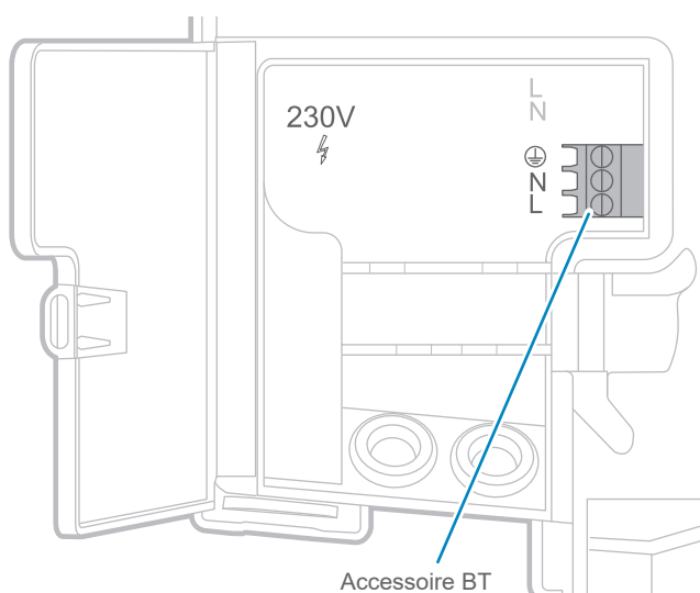
fig. 17 - Borniers BT
