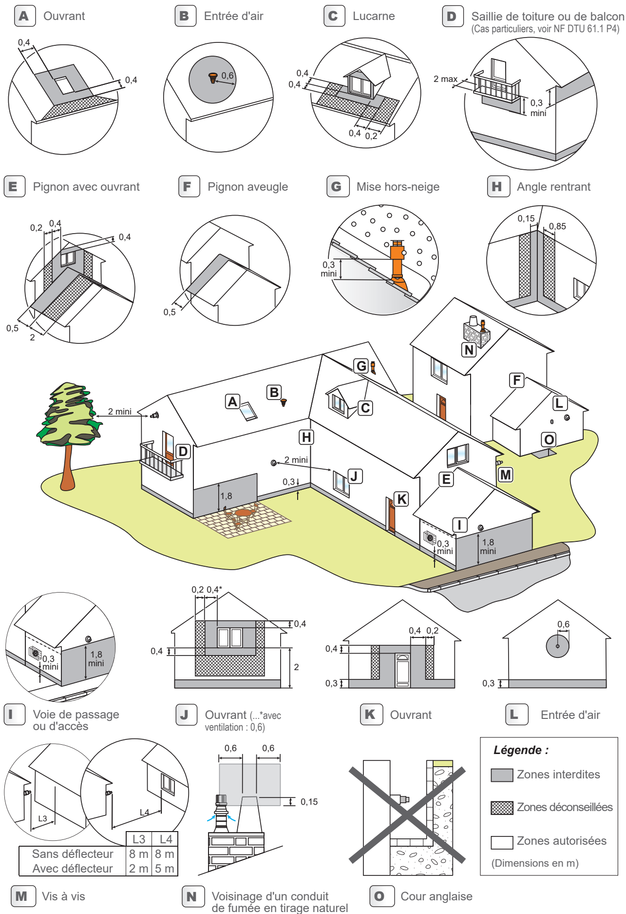
fig. 10 - Implantation du terminal (C13, C33)
