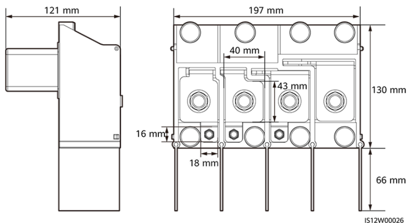
Figure 5-14 Dimensions du bornier CA
