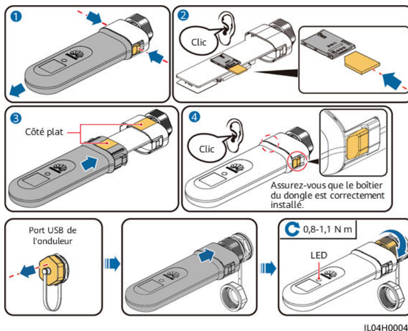
Figure 5-35 Installation du Smart Dongle 4G (SDongleB-06)
