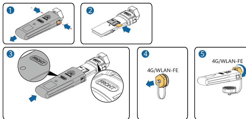
Figure 5-34 Installation du Smart Dongle 4G (SDongleA-03)
