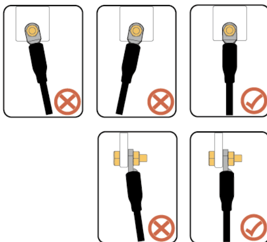
Figure 5-11 Exigences de câblage
