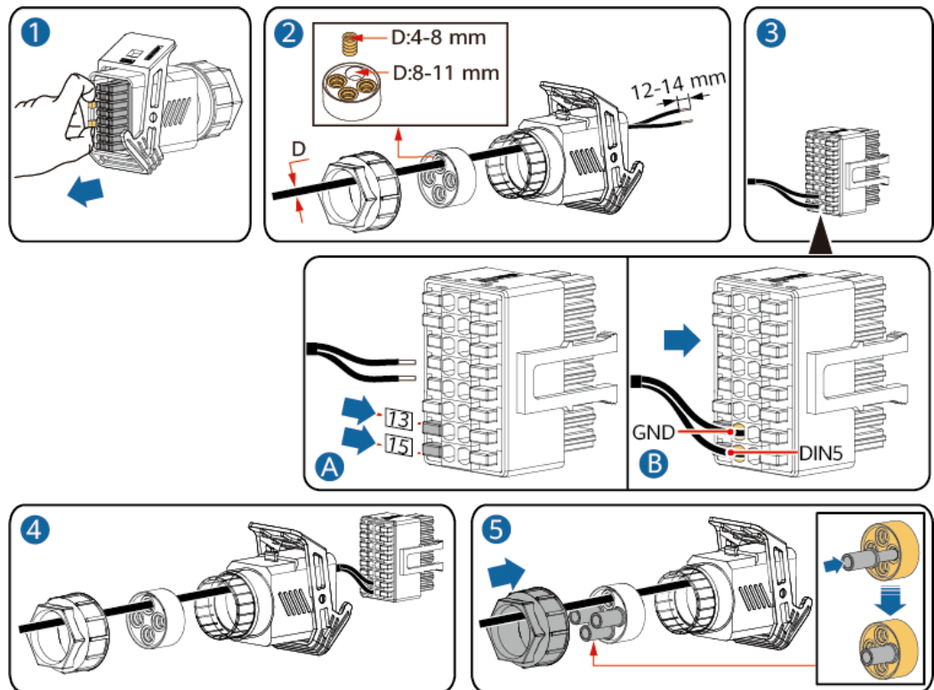
Figure 5-31 Installation du câble
