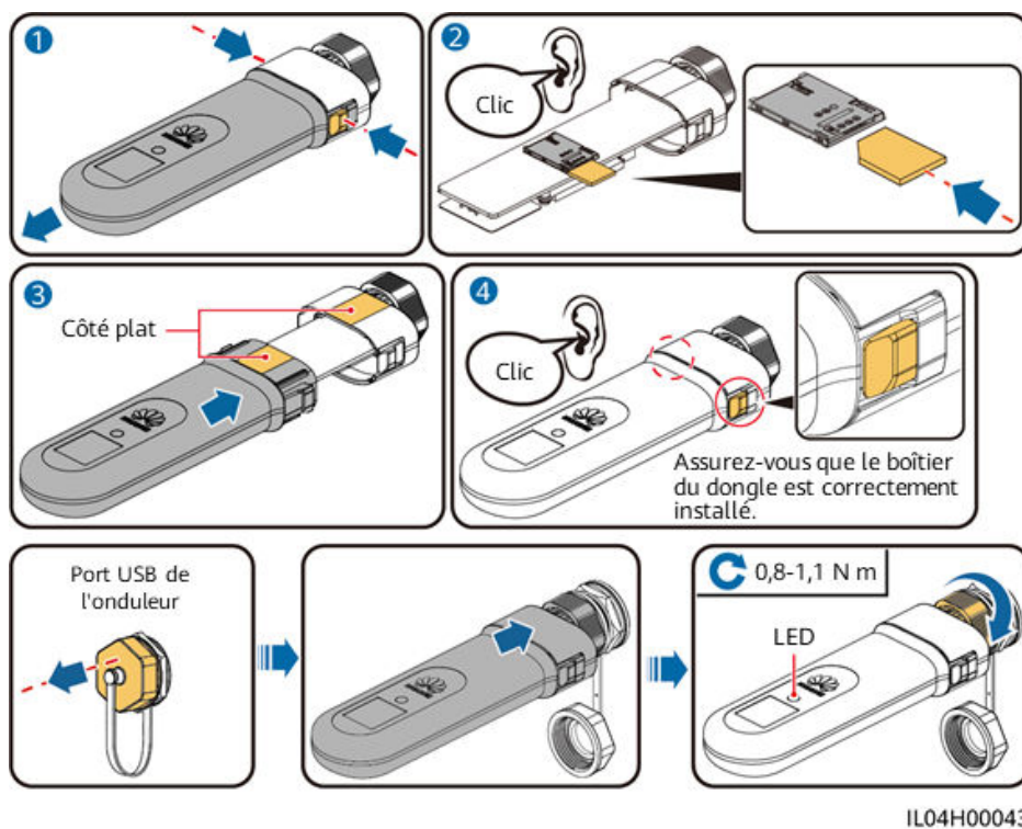
Figure 5-16 Installation du Smart Dongle 4G (SDongleB-06)
