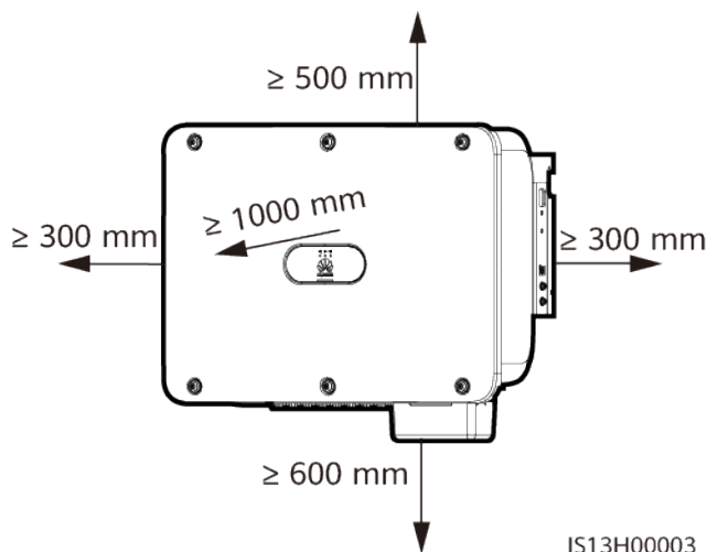
Figure 4-2 Distances
