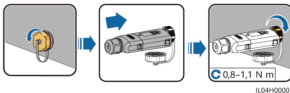
Figure 5-17 Installation du Smart Dongle WLAN-FE (communication WLAN)
