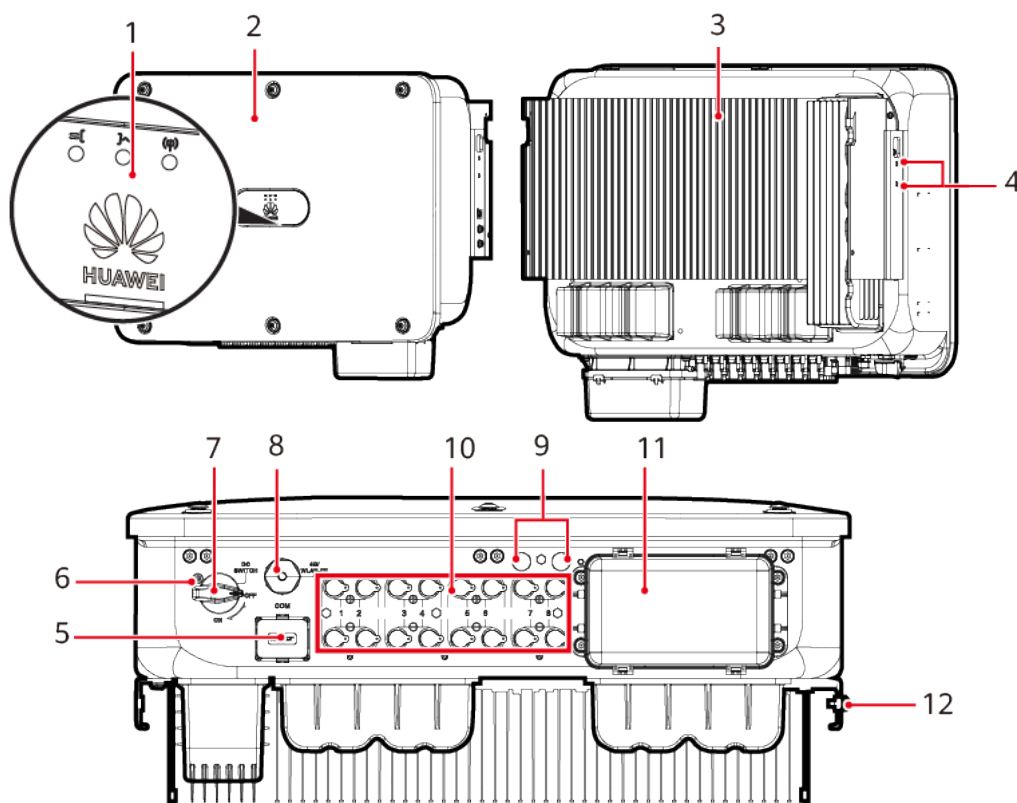
Figure 2-4 Apparence
