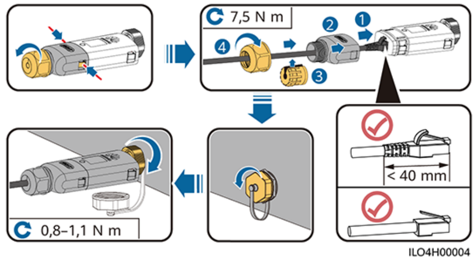
Figure 5-18 Installation du Smart Dongle WLAN-FE (communication FE)
