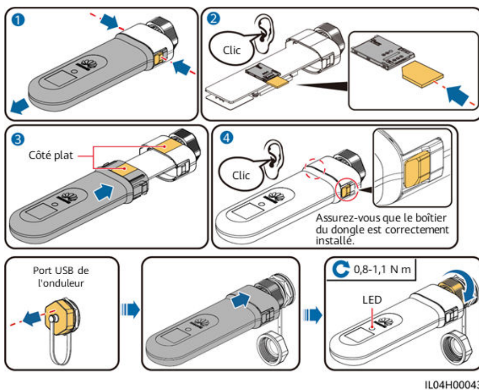
Figure 5-15 Installation du Smart Dongle 4G (SDongleB-06)
