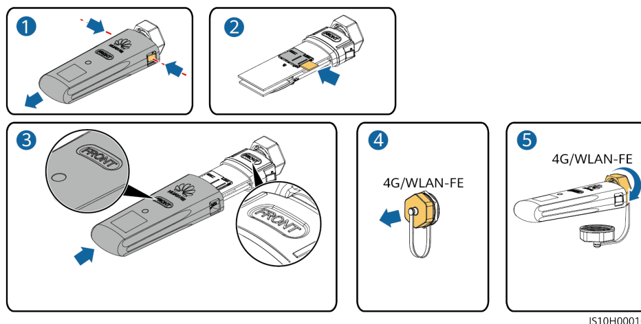
Figure 5-14 Installation du Smart Dongle 4G (SDongleA-03)
