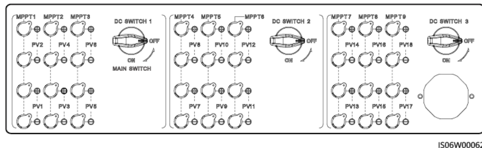
Figure 5-15 Bornes DC
