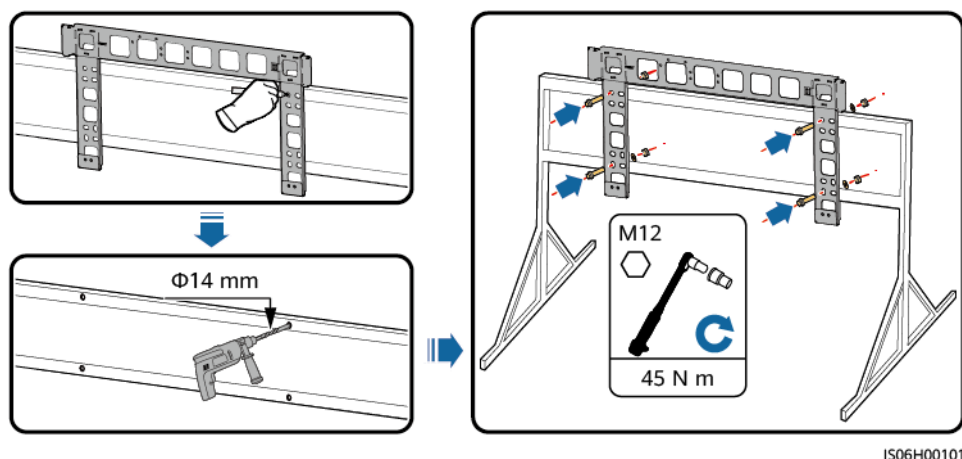
Figure 4-9 Installation du support de montage
