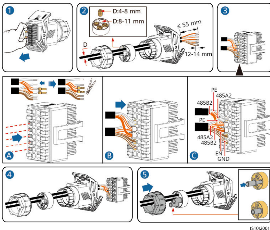
Figure 5-34 Installation des câbles
