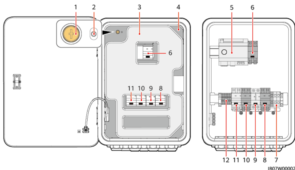
Figure 2-9 Compartiment de maintenance et bornes de raccordement
