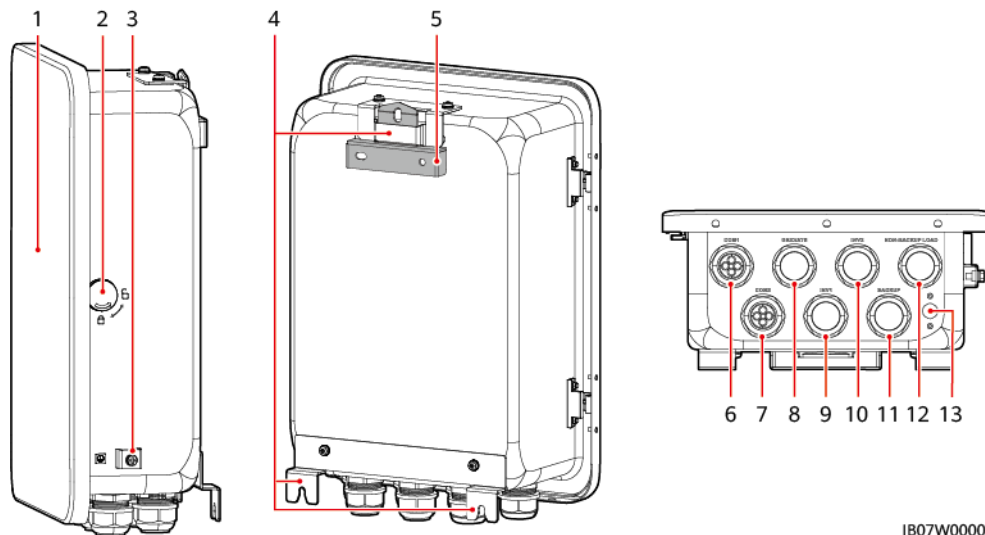
Figure 2-8 Aspect visuel et ports
