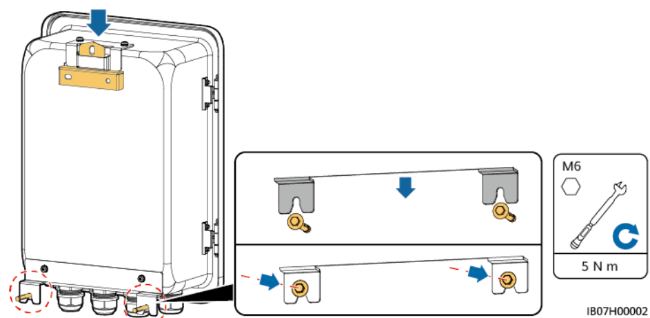
Figure 4-6 Installation du SmartGuard
