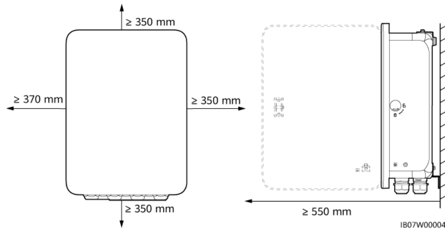
Figure 4-2 Distances
