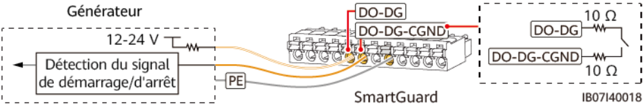
Figure E-1 Signal de Generator Control
