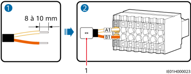
Figure 5-10 Raccordement des câbles de communication RS485
