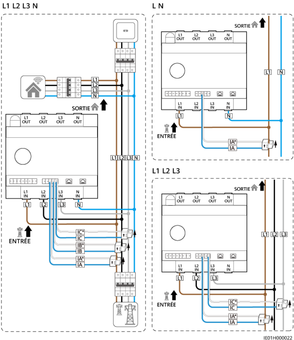
Figure 5-8 Connexion CT externe (courant > 63 A)
