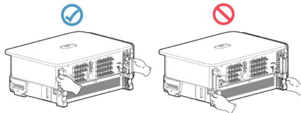
Figure 4-9 Positions de levage
