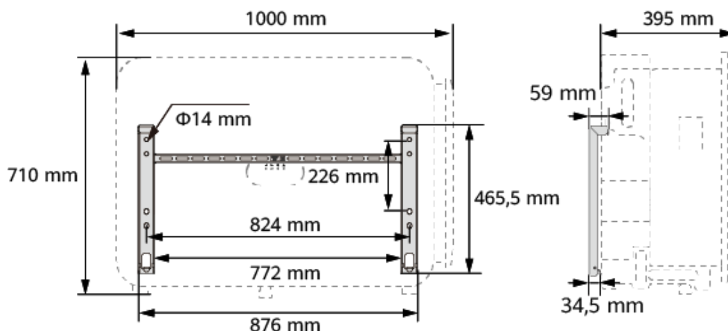
Figure 4-1 Dimensions
