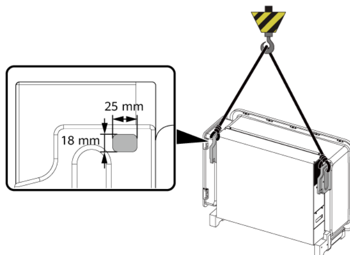
Figure 4-10 Levage
