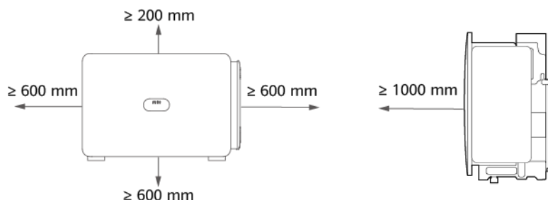
Figure 4-2 Distance
