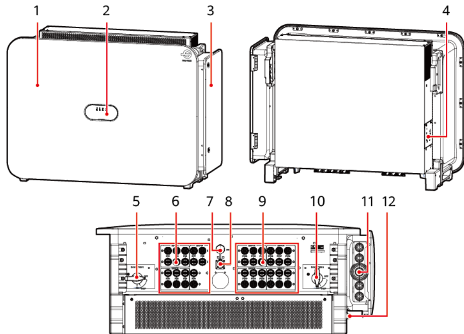
Figure 2-7 Aspect visuel
