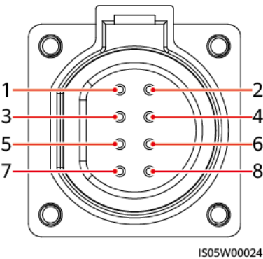
Figure 5-18 Port de communication
