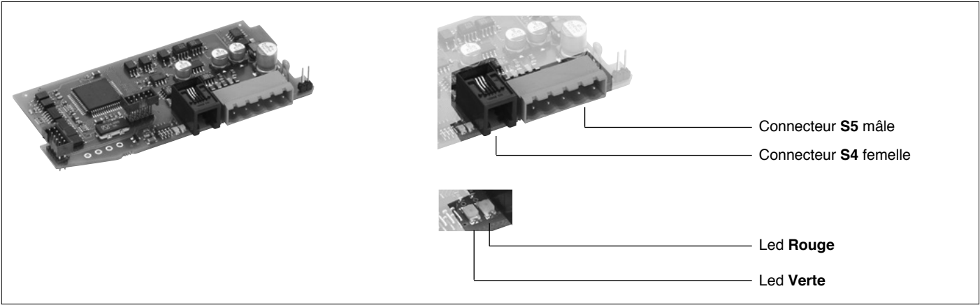
Figure 26 Port2: Interface Fieldbus Modbus RTU/DeviceNet
